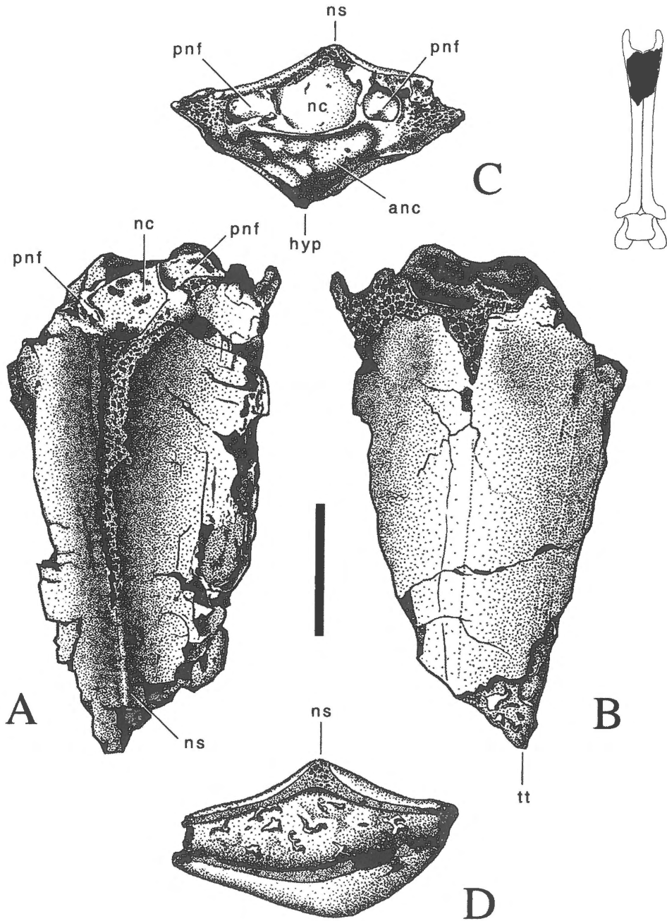
Figure 2. Azhdarchidae indet. from the Upper Cretaceous of La Solana (Tous area, Spain). Scale bar equals 20 mm. Anterior end of cervical vertebra (MPV TT48) in dorsal (A), ventral (B), anterior (C), and posterior (D) views. Inset shows position of fragment in the complete element. anc = anterior cotyle; hyp = hypapophysis; nc = neural canal; ns = neural spine; pnf = pneumatic foramen; tt = trabecular tissue.
