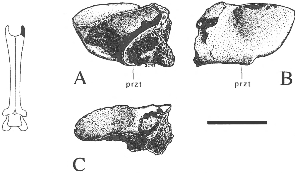
Figure 4. Azhdarchidae indet. from the Upper Cretaceous of La Solana (Tous area, Spain). Scale bar equals 20 mm. Right prezygapophysis (MGUV 3209) in medial (A), lateral (B) and dorsal (C) views. Inset shows position of fragment in the complete element. przt = prezygapophysial tubercle.
