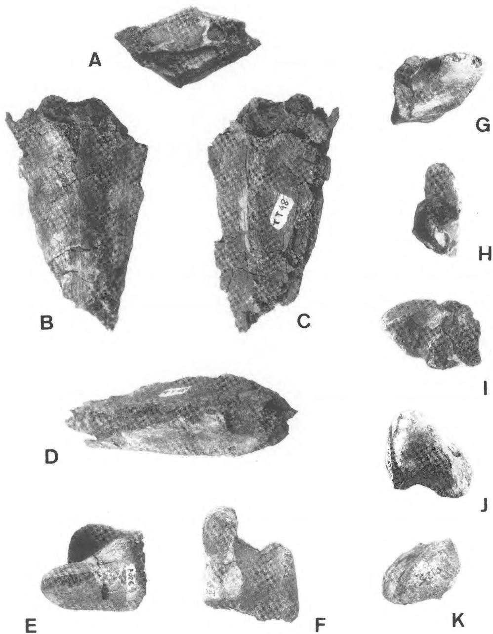
Plate I. Postcranial remains of Azhdarchidae indet. from the Upper Cretaceous of La Solana (Tous area, Spain). A–D: anterior end of mid-series cervical vertebra (MPV TT48) in anterior (A), ventral (B), dorsal (C) and right lateral (D) views, \times 0.8 . E–F: anterior end of mid-series cervical vertebra (MGUV 3207) in left lateral (E) and dorsal (F) views, \times 0.85 . G–I: right prezygapophysis (MGUV 3209) in right lateral (G), dorsal (H) and medial (I) views, \times 0.85 . J: right postexapophysis of cervical vertebra (MGUV 2194) in dorsal view, \times 0.85 . K: left postexapophysis of cervical vertebra (MGUV 3210) in dorsal view, \times 0.85 .
