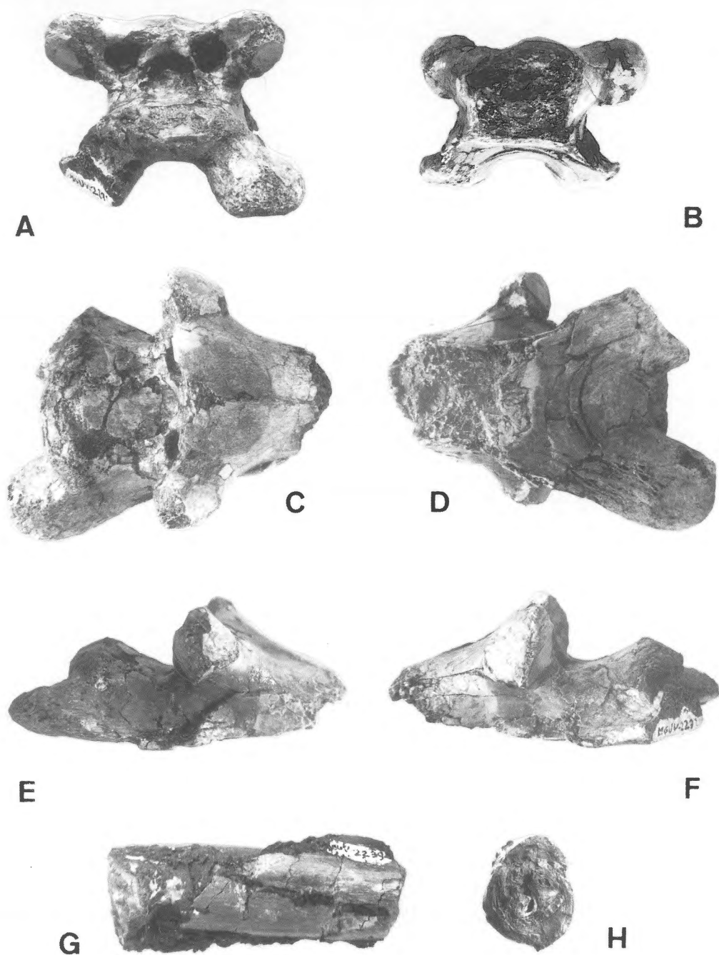
Plate II. Postcranial remains of Azhdarchidae indet. from the Upper Cretaceous of La Solana (Tous area, Spain). A–F: ?sixth cervical vertebra (MGUV 2271) in posterior (A), anterior (B), dorsal (C), ventral (D), right lateral (E), and left lateral (F) views, \times 0.75 . G–H: fragmentary limb bone (MGUV 2239) in ?dorsal (G) and ?proximal (H) views, \times 0.85 .
