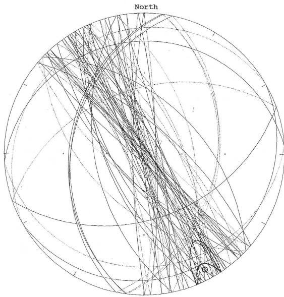
Figure 6. Great-circle trends from Group 1 dykes (39 specimens) by AF-demagnetization. Although scattered, the great circles clearly define a magnetic cross-over direction around (D, I) = (145^\circ, -12^\circ) .
