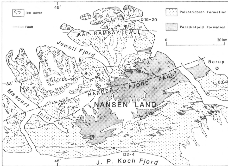
Figure 3. Geology of Nansen Land. Heavy lines (—) are major faults. The dykes are indicated as thin lines (not all dykes are shown). Dyke sampling areas are shown with dots, the sites clustering in three groups (D2-4, D5-14, and D15-20). The oldest dykes (Group 1, trending N-S) dominate north of the Kap Ramsay Fault, the dykes of intermediate age (Group 2, NW-SE) dominate between the Harder Fjord Fault and Kap Ramsay Fault, and the youngest dykes (Group 3, E-W) dominate south of the Harder Fjord Fault.
