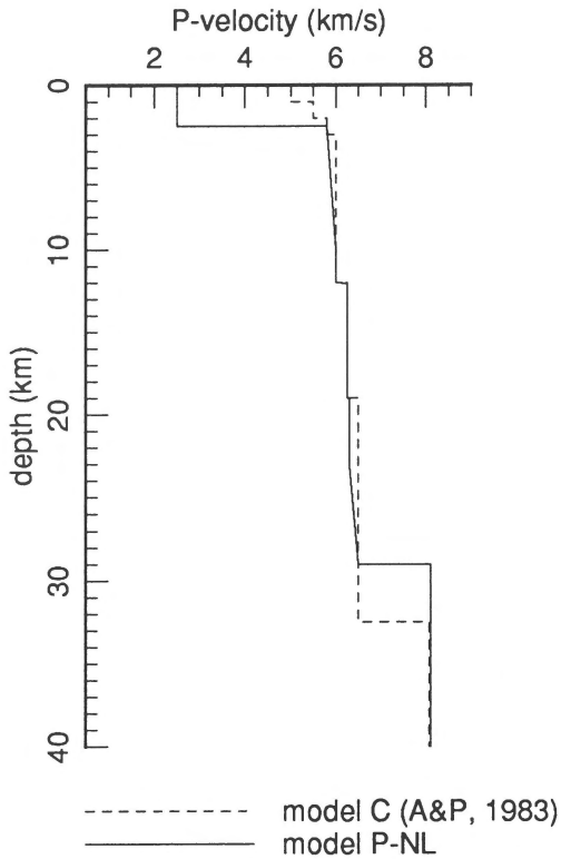
Fig. 3. P-velocity structure used for the determination of the epicentral location (dashed line, model C of Ahorner & Pelzing, 1983), and for modelling the P-wave phases (solid line, model P-NL).
